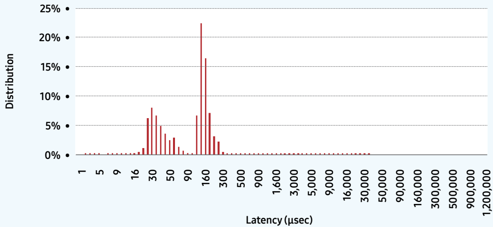
Figure 11: RocksDB Read Latency Distribution when data resides in PM1725a
