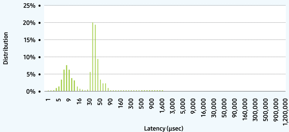
Figure 12: HeRocks Read Latency Distribution when data resides in Z-SSD
